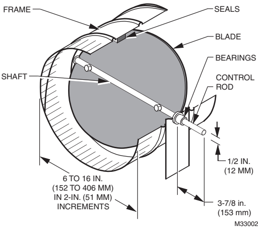
Fig. 1. D690 Dimensions.
