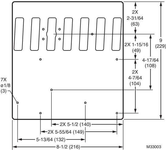
Fig. 2. D690 Actuator Mounting Plate Dimensions, in inches (mm).
