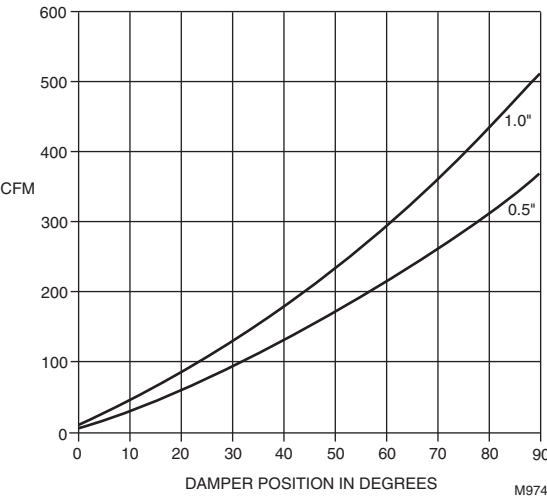
Fig. 3. 6-inch D690 flowrate vs. damper position.
